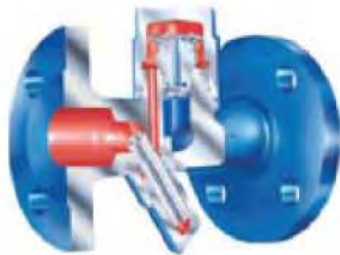
THERMOSTATIC STEAM TRAP GG25,GGG 40.3 C/S PN16, PN25, PN40
